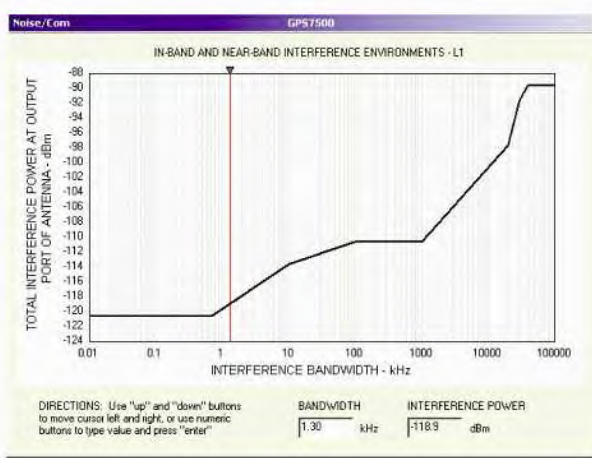
Interference Level vs. Interference Bandwidth
