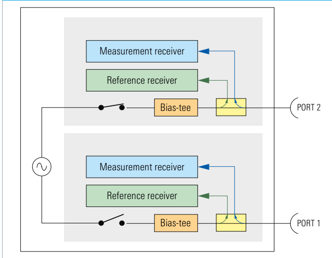
Block diagram of the R&S®ZVA two-port model
