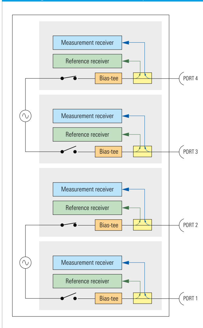
Block diagram of the R&S®ZVA four-port model
